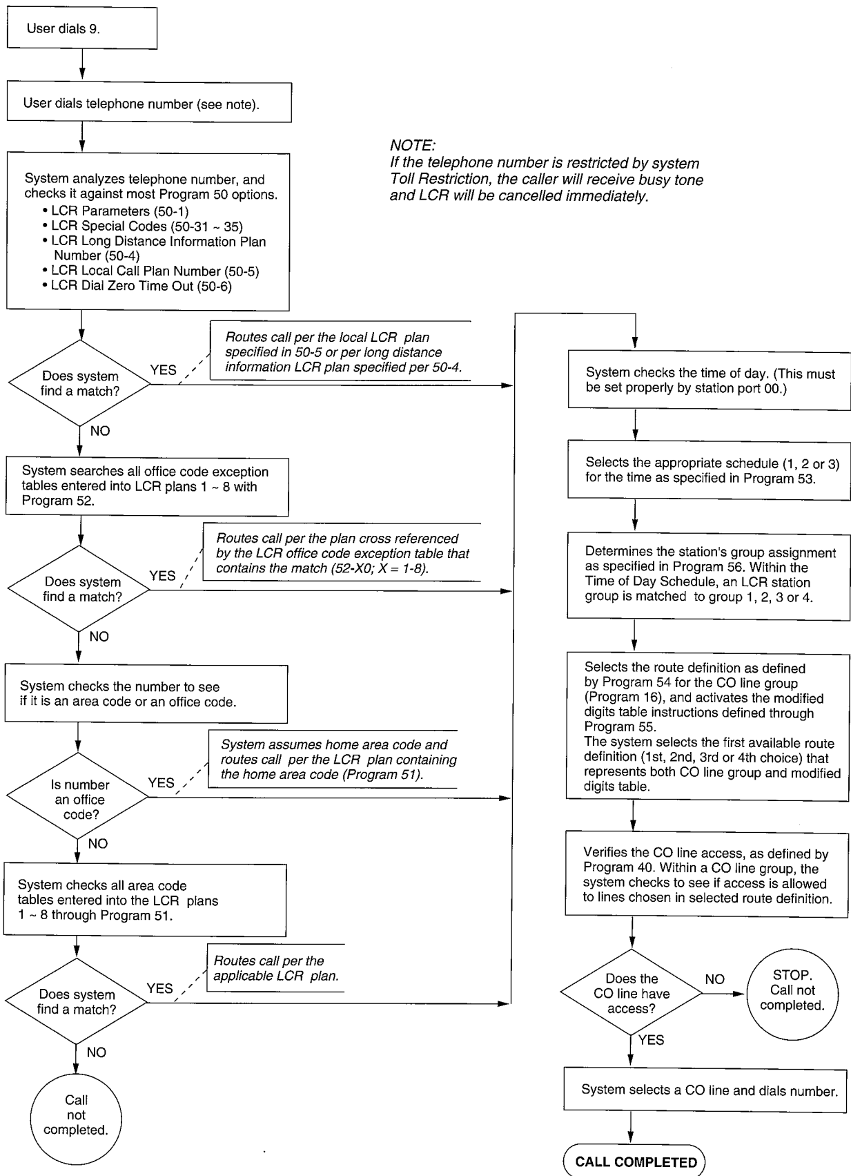
Figure 2-2 LCR OPERATIONAL BLOCK DIAGRAM
